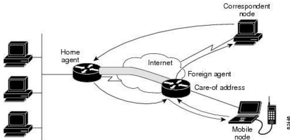
Figure 2 Packet Forwarding
